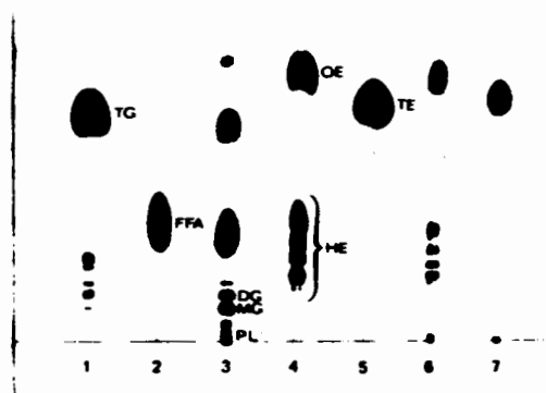
FIG. 3. Qualitative one-dimensional TLC in the solvent mixture hexane/diethyl ether/acetic (90:30:1) of sunflower oil (1), oleic acid (2), sunflower oil with taurocholate and lipase (3), SPE (4), TCCTE (5) and SPE (6) and TCCTE (7) with taurocholate and lipase. TG triglycerides, DG diglycerides, MG monoglycerides, FFA free fatty acids, PL phospholipids, OE octaesters, HE heptaesters, TE triesters.
